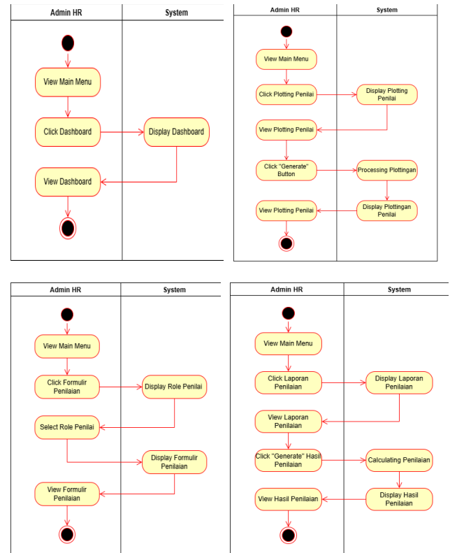
Figure 5. Activity Diagram
