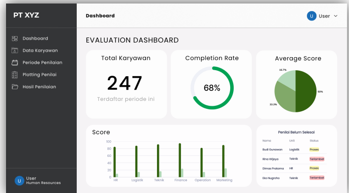
Figure 8. Dashboard Feature
